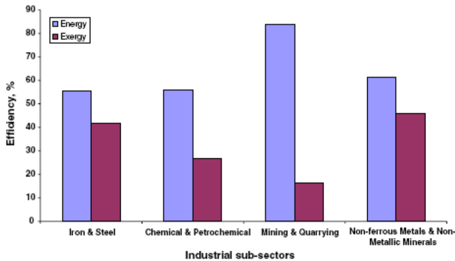
Fig. 3. Weighted mean efficiencies in the industrial sector, 1994–2003.
