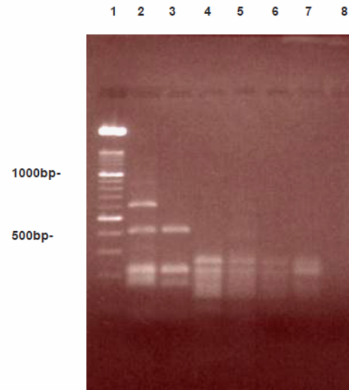
Figure 1: Agarose gel electrophoresis of amplified 16S rDNA of seven tentative Azospirillum isolates digested with restriction endonuclease AluI. Lane 1: 100bp ladder maker; Lanes 2–8: B12AM, B13SSP, B33CE, B34CE, B13SAF, B22PR10 and B12CCD10
