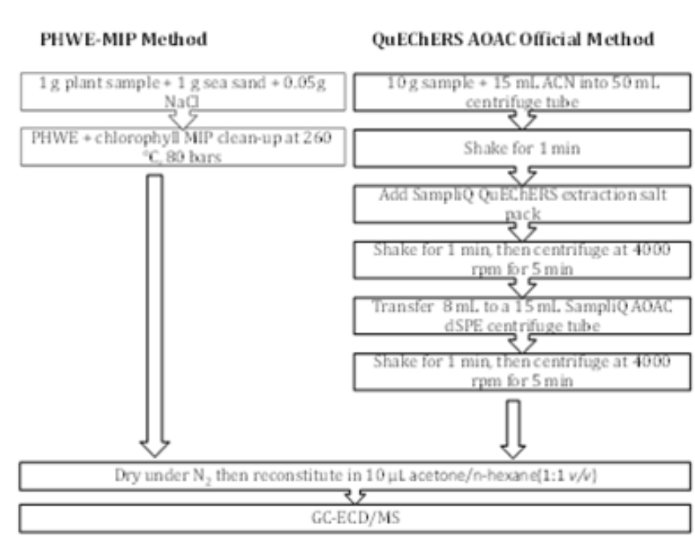
Figure 3. Comparison of the extraction scheme of QuEChERS method with PHWE-MIP.
