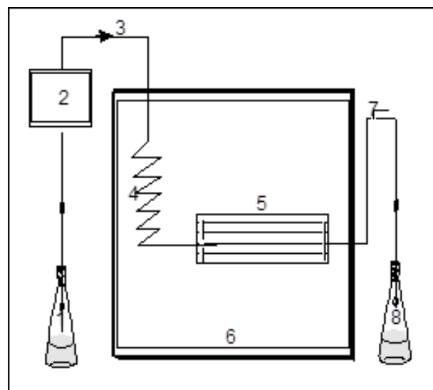
Figure 1. Schematic diagram of laboratory self - assembled PHWE system. 1. Solvent system 2. Pump 3. Flow direction 4. Preheating coil 5. Extraction cell 6. Gas chromatography oven 7. Back pressure regulator 8. Collecting flask.
