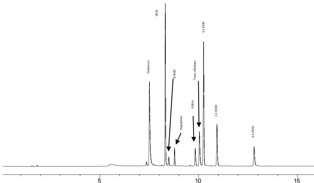
Figure 4. A chromatogram of pesticides detected from N. lotus when PHWE was combined with a chlorophyll MIP.
