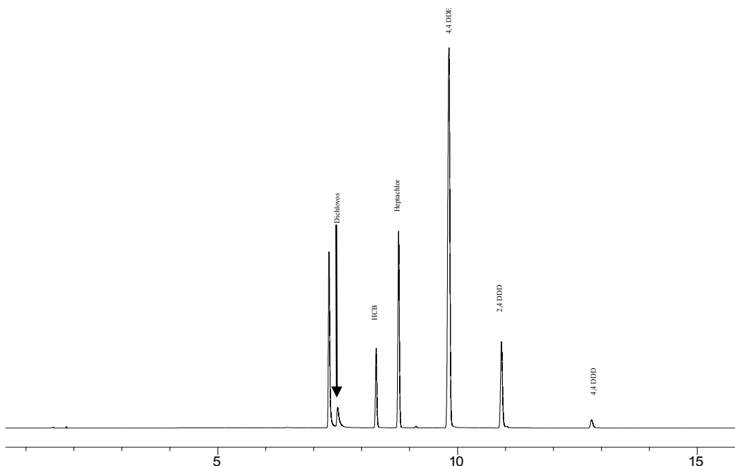
Figure 4. A chromatogram of pesticides detected from N. lotus when PHWE was combined with a chlorophyll MIP.
