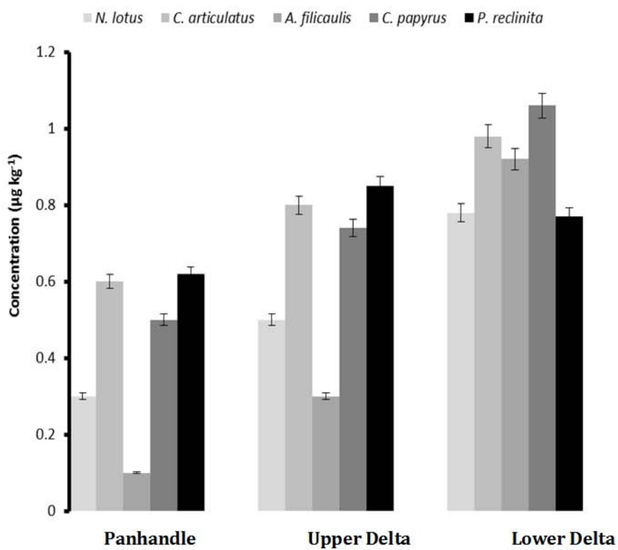
Figure 6. Concentration of 4,4DDE in different plants from all sampling regions. All other pesticides show a similar trend.
